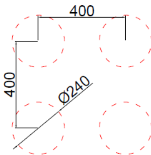
Figure 7. QMC6309 PCB footprint
