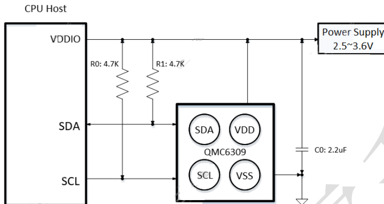
Figure 6. VDDIO is the same as VDD
